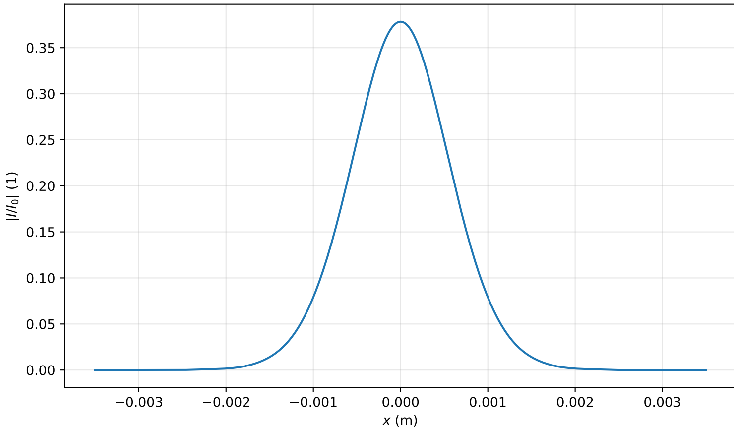
Intensity profile I(x, y = 0, z = 3.264m)/I_0 , P_{in}=0.3P_{cr} , artificial time
